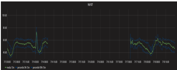
Figure 4. Breakage of microphone put in evidence by the signal interruption shown by the time history of sound pressure levels.
