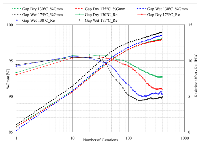
Figure 3. GPDA results of gap graded mixes.
