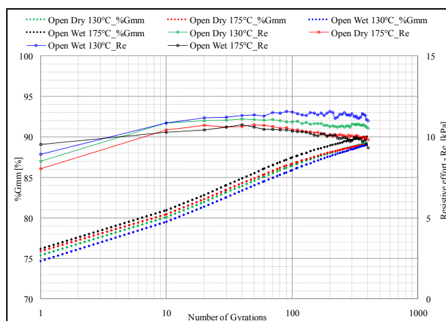
Figure 4. GPDA results of open graded mixes.
