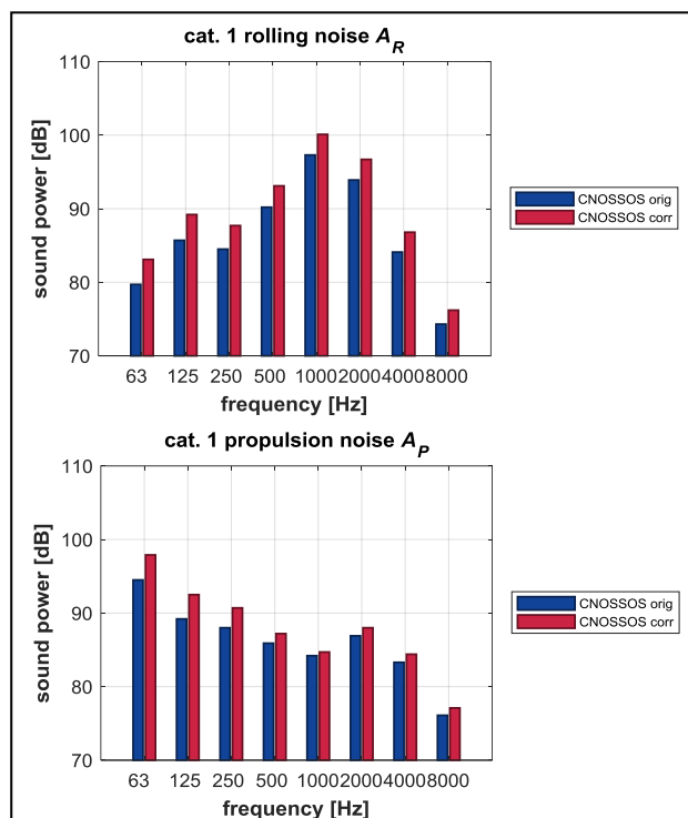
Figure 7: Corrected vs. original CNOSSOS-EU sound power coefficients for light motor vehicles; top : rolling noise A_R , bottom : propulsion noise A_P
